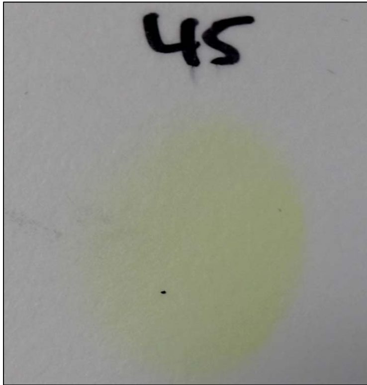
Chemical spot test #45, Sulfuric Acid (77%) and Nitric Acid (70%), equal parts, Rating 2, color change
