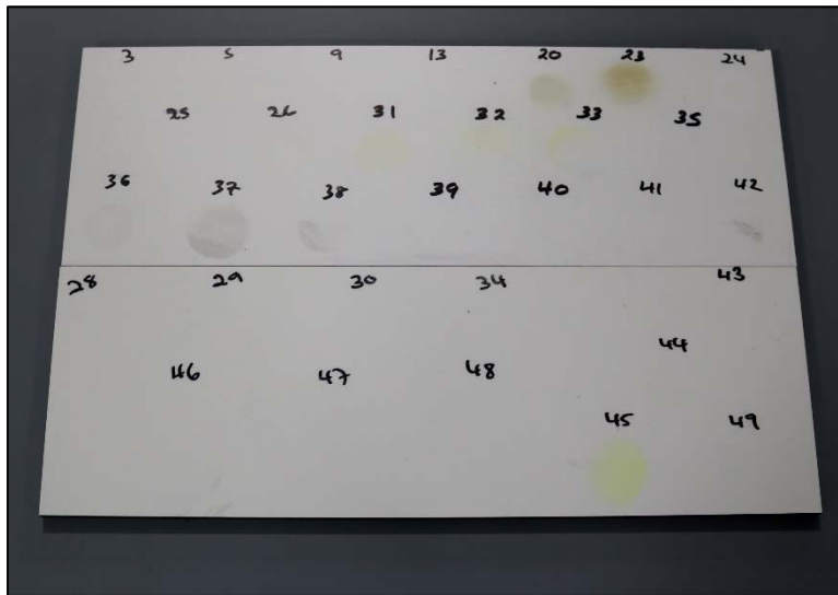
Chemical Spot Test Non-volatile after Exposure, White Sample
