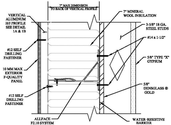
4 MAXIMUM INSULATION CAVITY DEPTH
