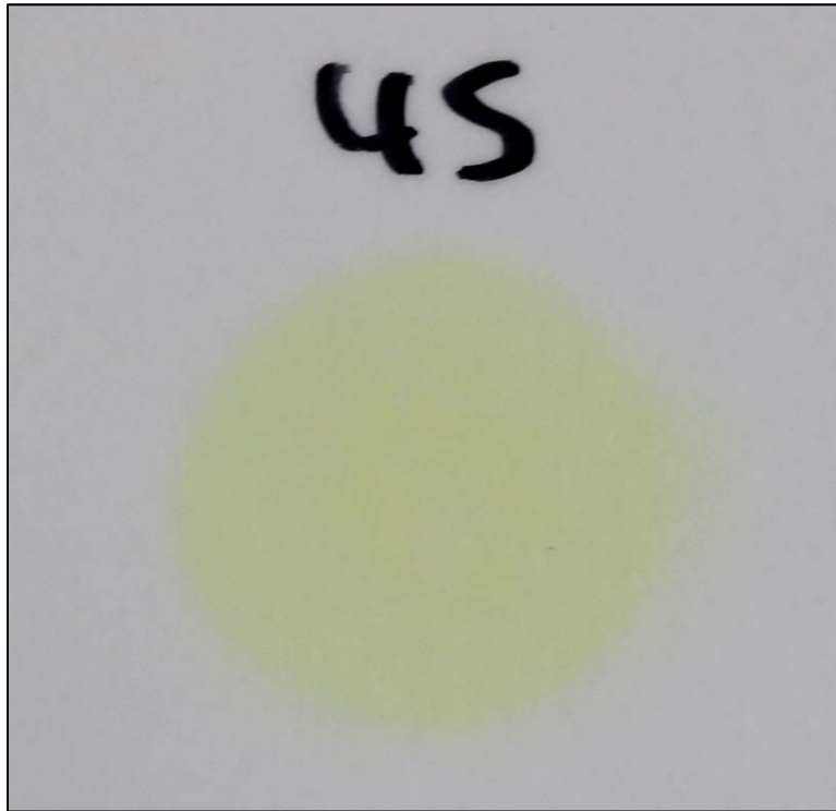
Chemical spot test #45, Sulfuric Acid (77%) and Nitric Acid (70%), equal parts, Rating 2, Color change
