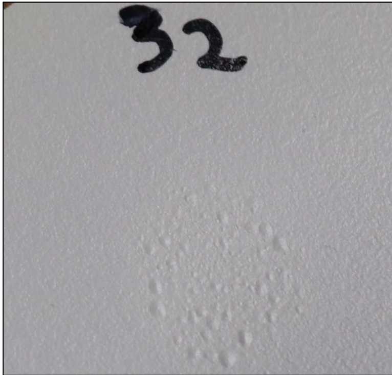
Chemical spot test #32, Nitric Acid (30%), Rating 3, Surface swelling
