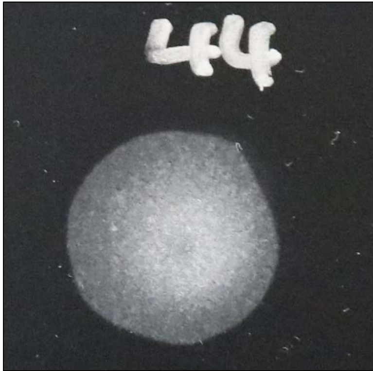
Chemical spot test #44, Sulfuric Acid (96%), Rating 2, Gloss change, Color change
